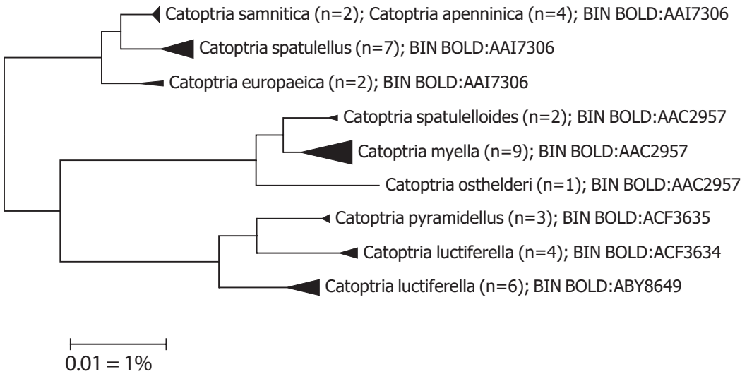
Figure 27. Neighbor-Joining tree (Kimura 2 parameter, built with MEGA 6; cf. Tamura et al. 2013) of species of the Catoptria permutatella species group from Italy. The width of the triangles represents the sample size, and the depth the genetic variation within the cluster. Source: DNA Barcode data from BOLD (Barcode of Life Database, cf. Ratnasingham and Hebert 2007).
